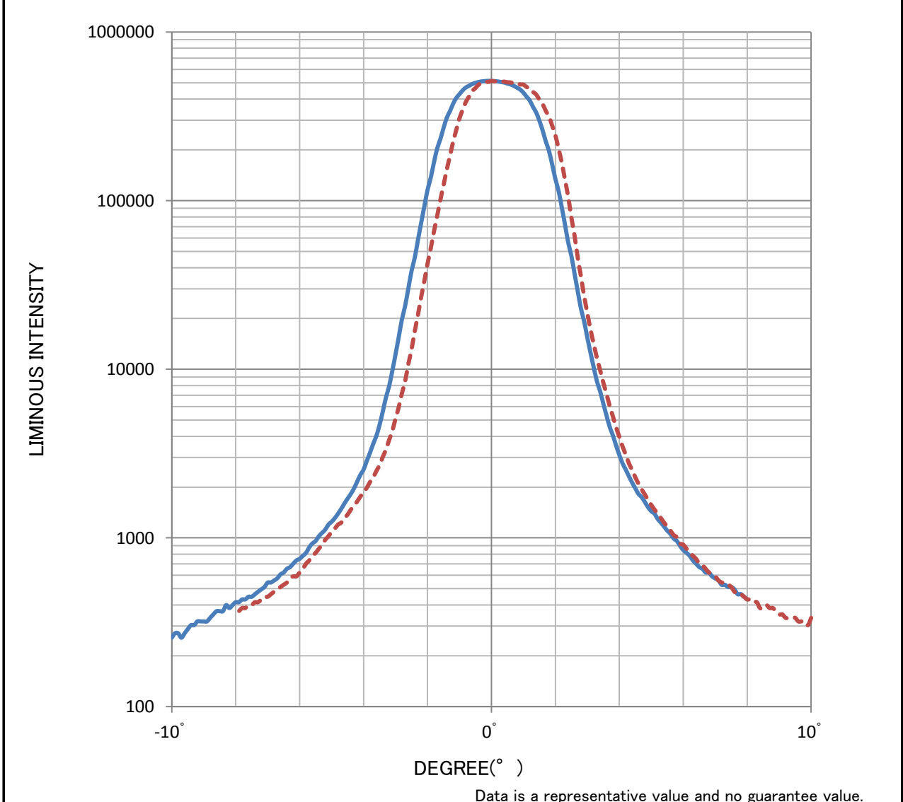
DISTRIBUTION CURVE OF LUMINOUS INTENSITY (UNIT : cd/1000lm)
