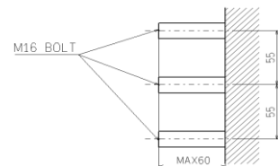
INSTALLATION BOLT
